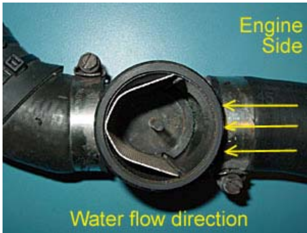
Place in correct direction (stamped IN and OUT) and slide the unit in place.
